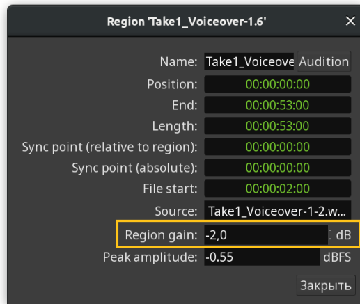
Fig. 53.1 - Region Properties
