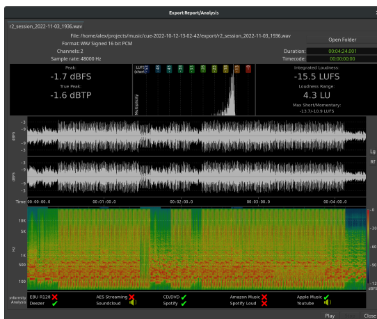
Fig. 45.3 - The Export Report/Analysis window
