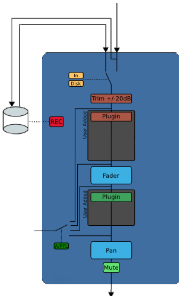
Fig. 71.16 - Typical signal routing in a channel strip.
