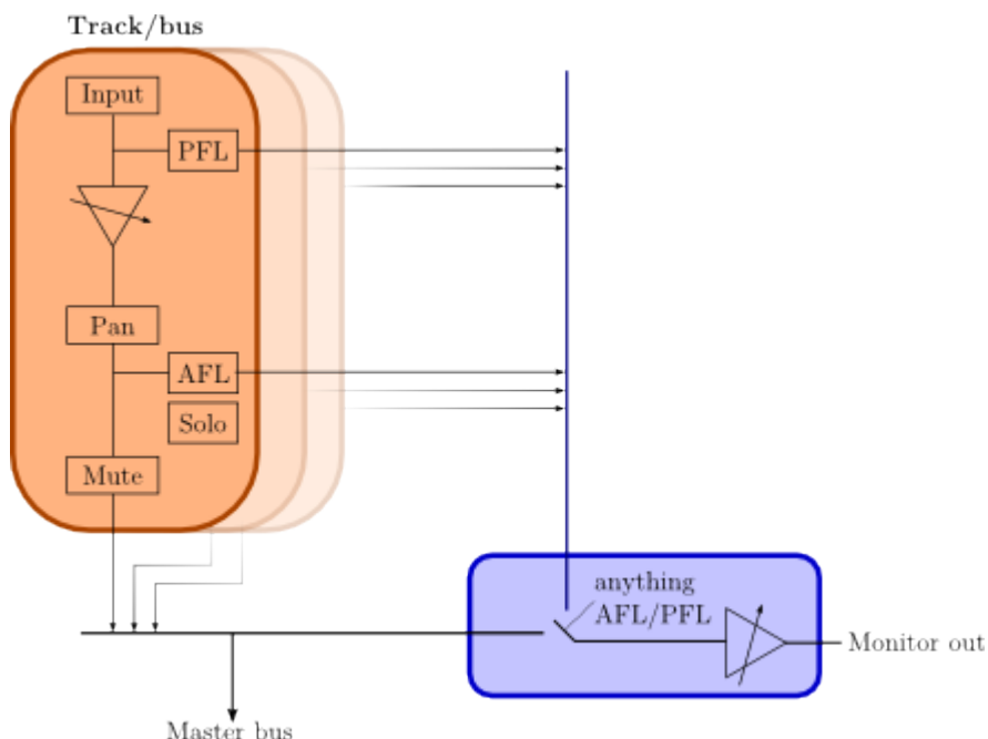
Fig. 71.21 - Mute/solo signal flow
