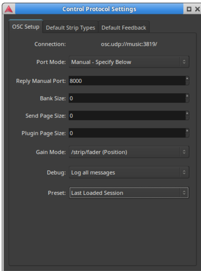
Fig. 82.1 - The OSC configuration dialog
