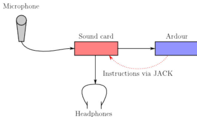
Fig. 42.2 - Hardware Monitoring
