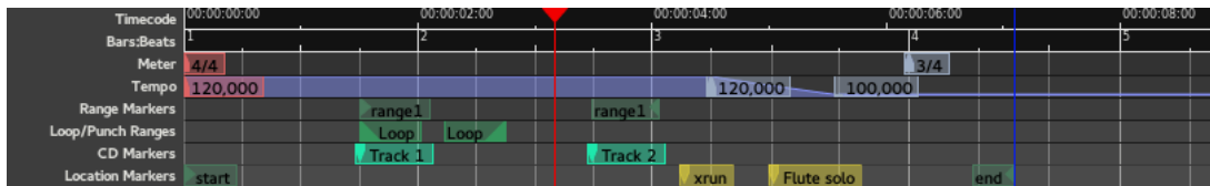
Fig. 21.1 - Ardour's Ruler
