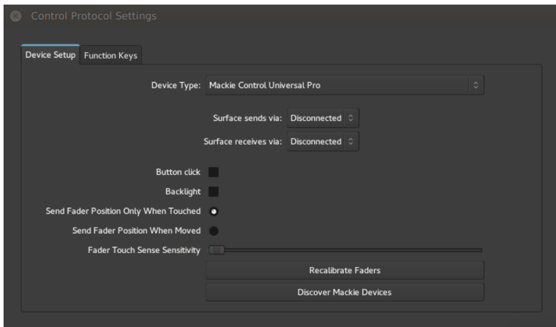
Fig. 83.1 - The Mackie Control Setup Dialog
