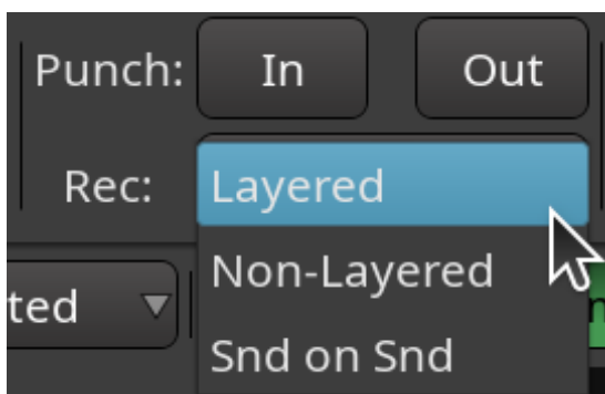
Fig. 34.7 - Layering switch
