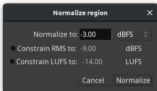
Fig. 53.3 - Normalize Region
