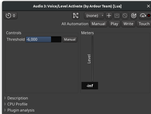
Fig. 76.5 - Voice/Level Activate
