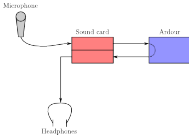
Fig. 42.3 - Software Monitoring
