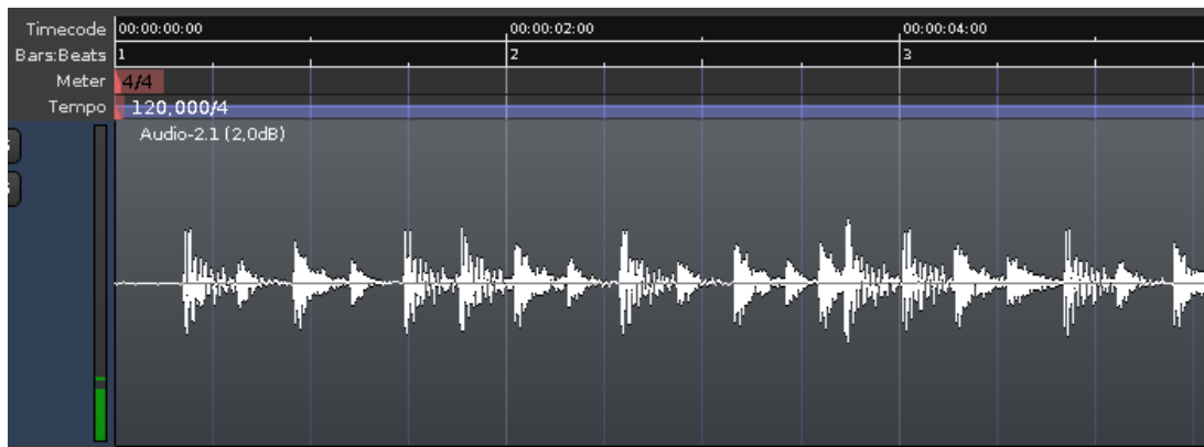
Fig. 70.3 - Initial state.
