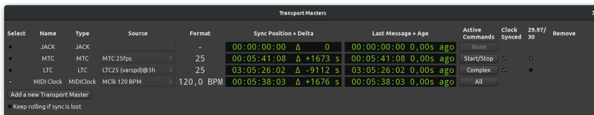
Fig. 6.4 - Transport Masters
