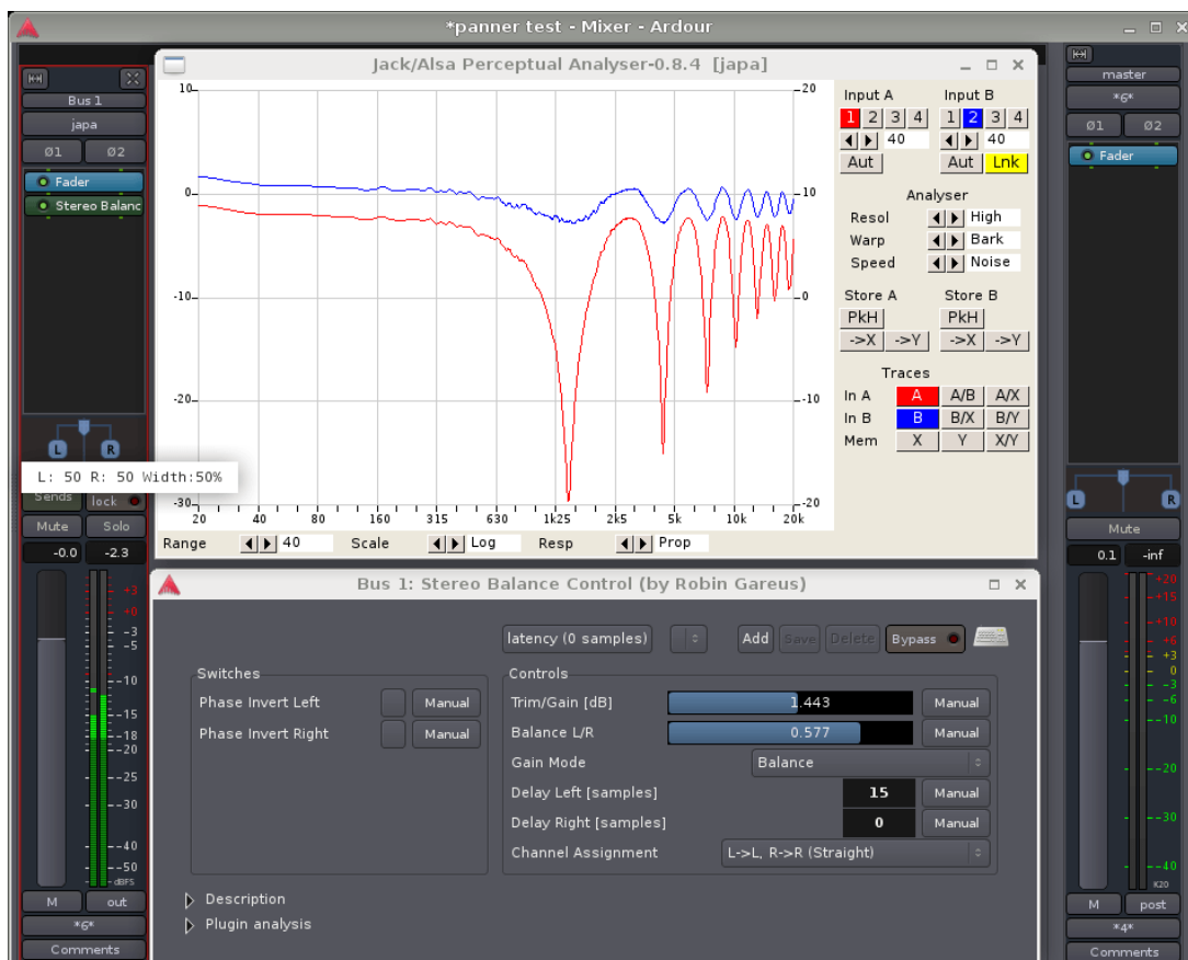
Fig. 71.26 - Stereo panner with ORTF half width
