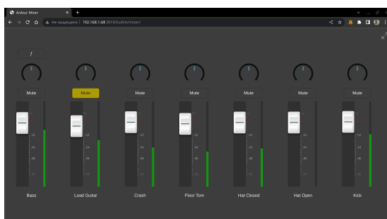
Fig. 94.2 - Mixer view in WebSockets Server
