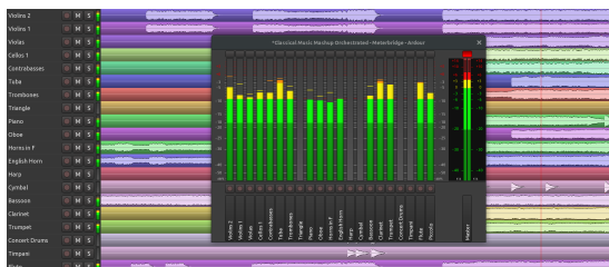
Fig. 71.4 - Meterbridge window
