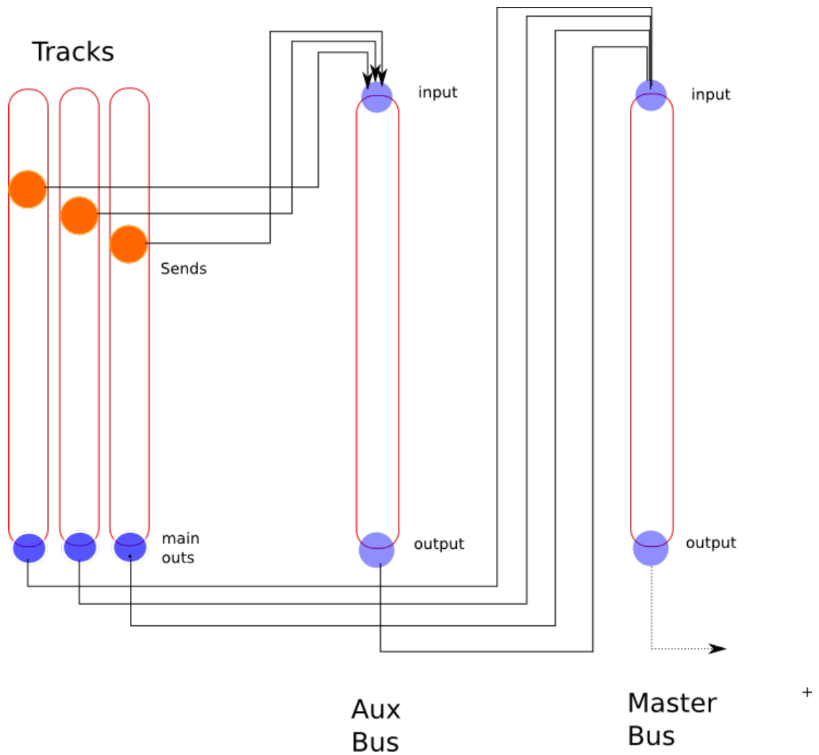
Fig. 58.7 - Aux signal routing
