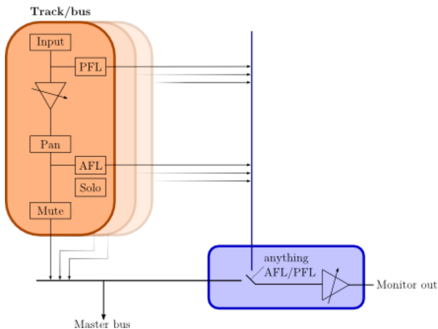
Fig. 58.15 - Mute/solo signal flow
