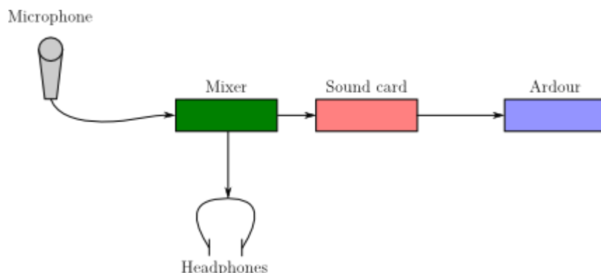
Fig. 39.1 - External monitoring
