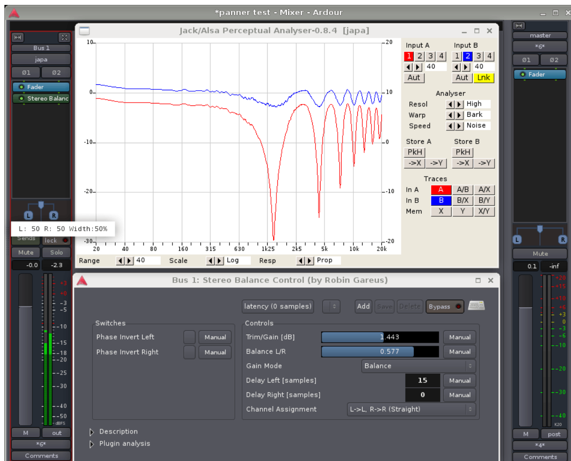
Fig. 58.20 – Stereo panner with ORTF half width
