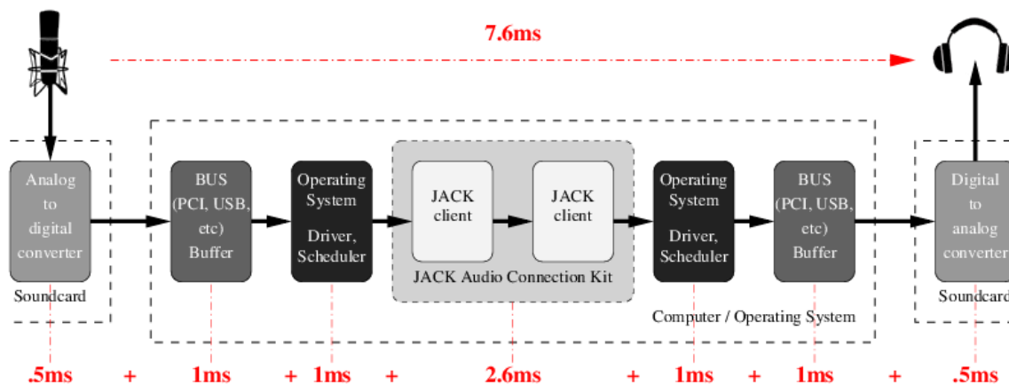
Fig. 7.1 - Latency chain
